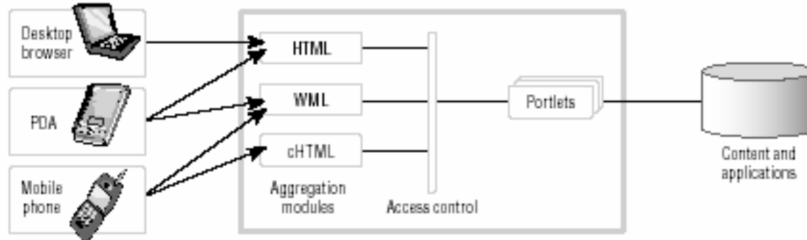
Figure 4. Page content aggregation
